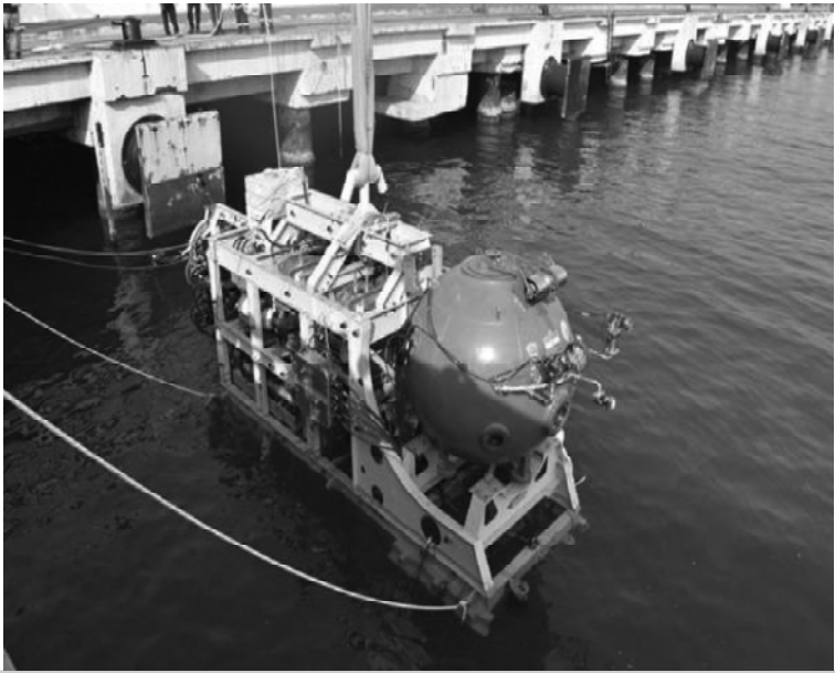
Unmanned, without buoyancy module
